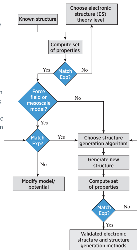
Figure 3-6. Decision Tree Diagram of Structure Determination and Computing.
