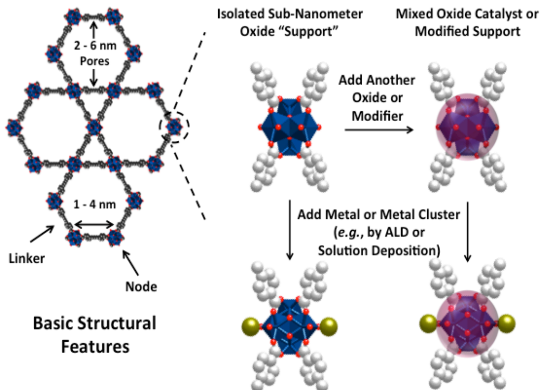
Figure 3-1. Metal and Metal-Oxide Catalyst of Atomic Precision Anchored at a Support for Natural Gas Conversion Catalysis. In order to model full catalytic processes of this type, exascale resources will be needed (Source: ICDC 2016).
