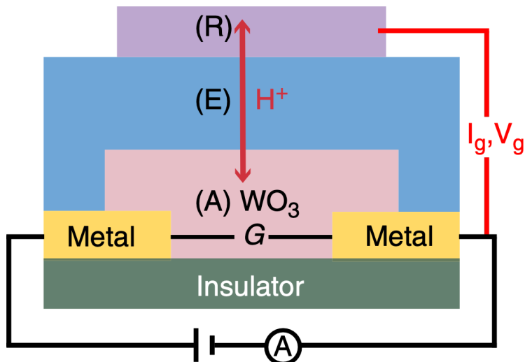
Conductivity switch in H-doped WO 3
