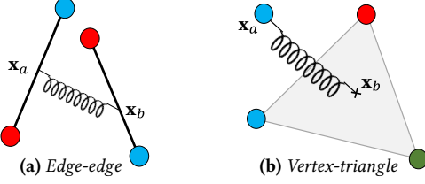
Fig. 4. Two collision types: (a) edge-edge can have at most two pairs and (b) vertex-face can have at most one pair with the same color, since vertices on the same side of a collision must have different colors.
