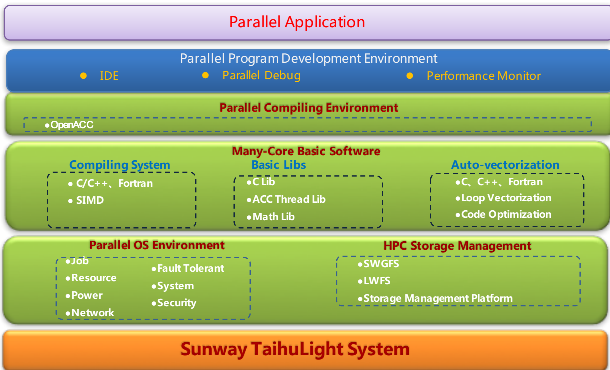
Figure: Sunway TaihuLight Software Stack
