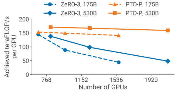
Figure 10: Throughput per GPU of PT-D-P and ZeRO-3 for two different GPT models (the 175B GPT-3 model is shown with dotted lines, and the 530B model is shown with solid lines). Global batch sizes are fixed and ZeRO-3 is used without any model parallelism.
