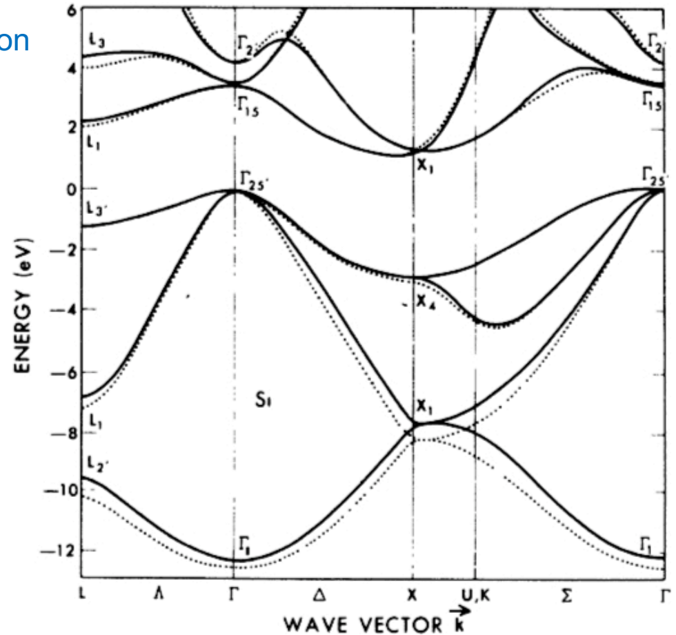
Kohn-Sham energy
