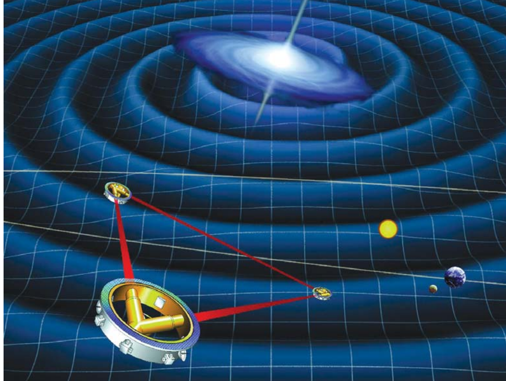
FIGURE 2. THE LASER INTERFEROMETER SPACE ANTENNA (LISA) could detect gravitational waves that have frequencies ranging from 0.1 mHz to 100 mHz. By way of comparison, the gravitational wave discovered with the Laser Interferometer Gravitational-Wave Observatory last February featured frequencies around 100 Hz. Spanning millions of kilometers, LISA will be by far the largest structure produced by humanity. It will be a lasting monument to our curiosity, ambition, and ingenuity. (Courtesy of NASA.)
