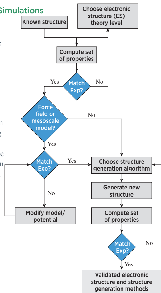
Figure 3-6. Decision Tree Diagram of Structure Determination and Computing (adapted from diagram available at microm-center.org/validation.html ).
